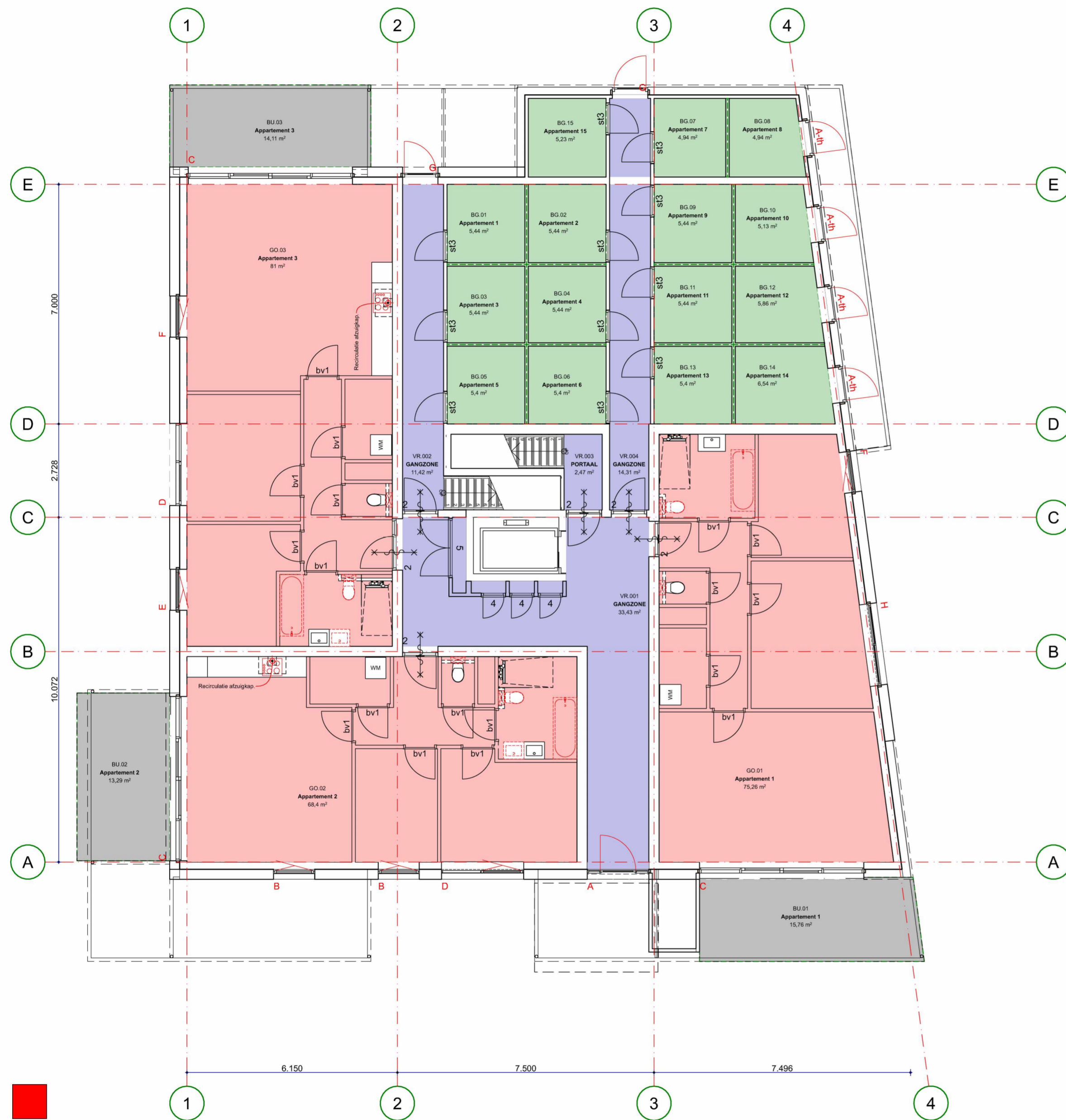
0. Begane grond
